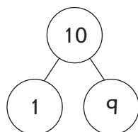
part-whole model
